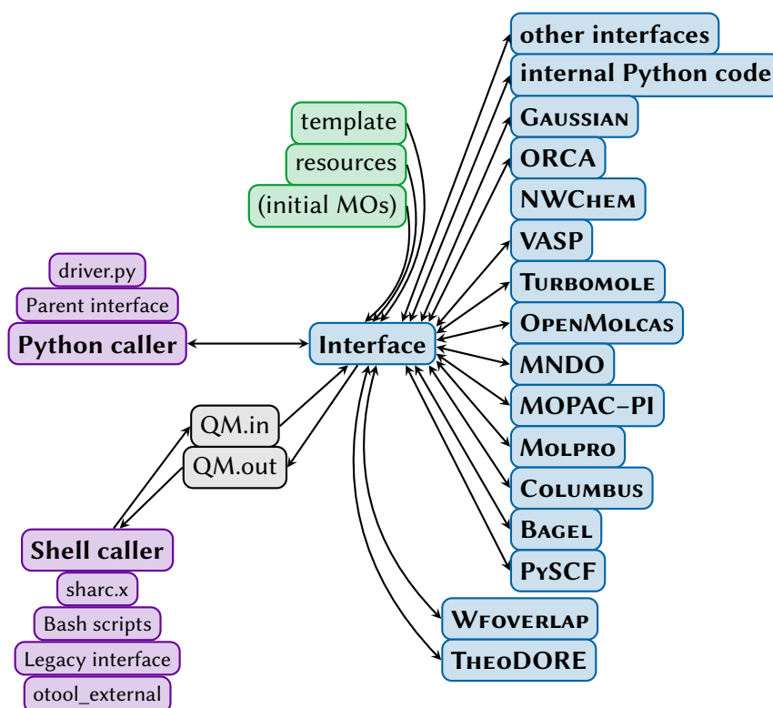
Figure 6.1: Communication between sharc.x , driver.py , the interfaces, and the quantum chemistry codes.
